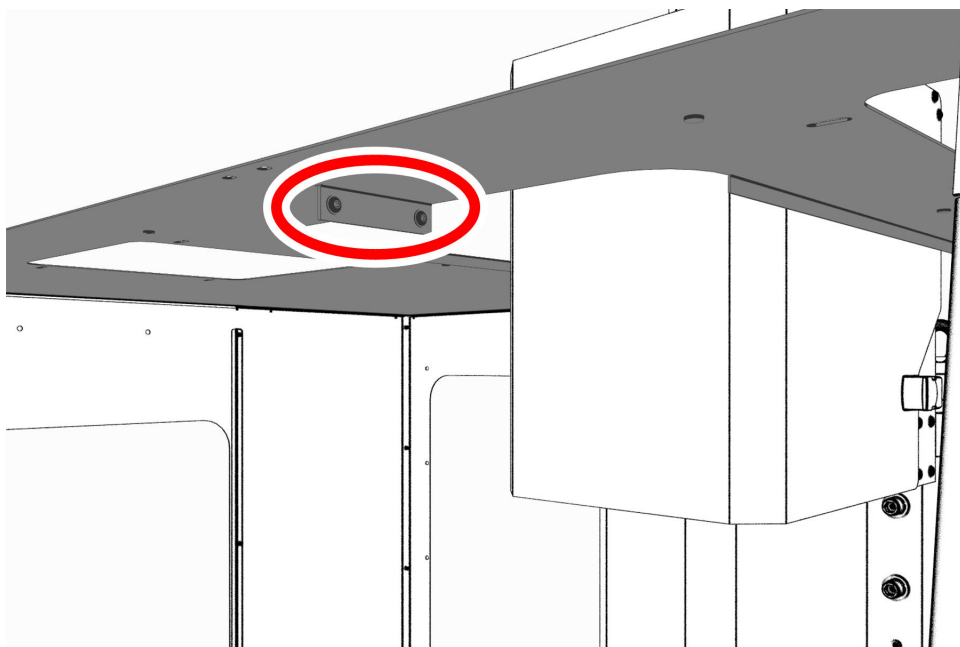
Figure 13: Left and right top panels connected.
