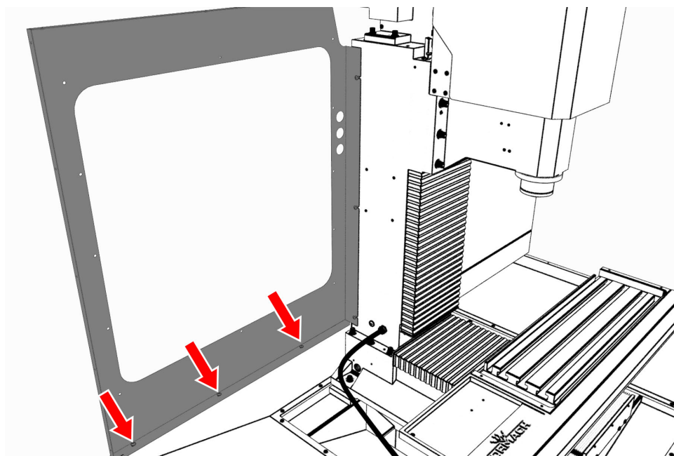
Figure 1: Left rear panel attached to the left chip pan.
