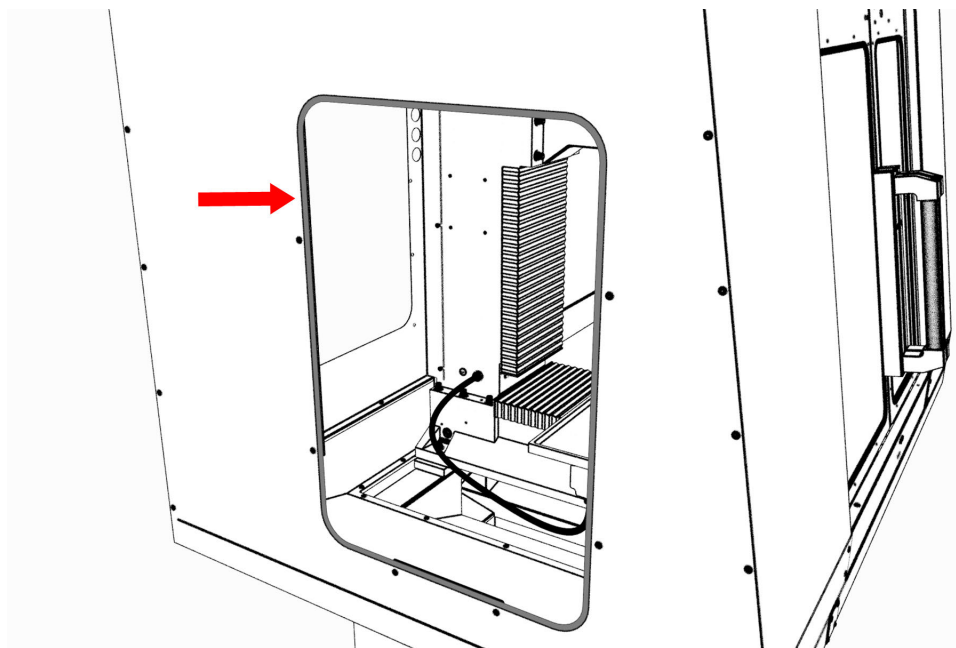
Figure 31: Rubber trim pushed onto the window opening.
