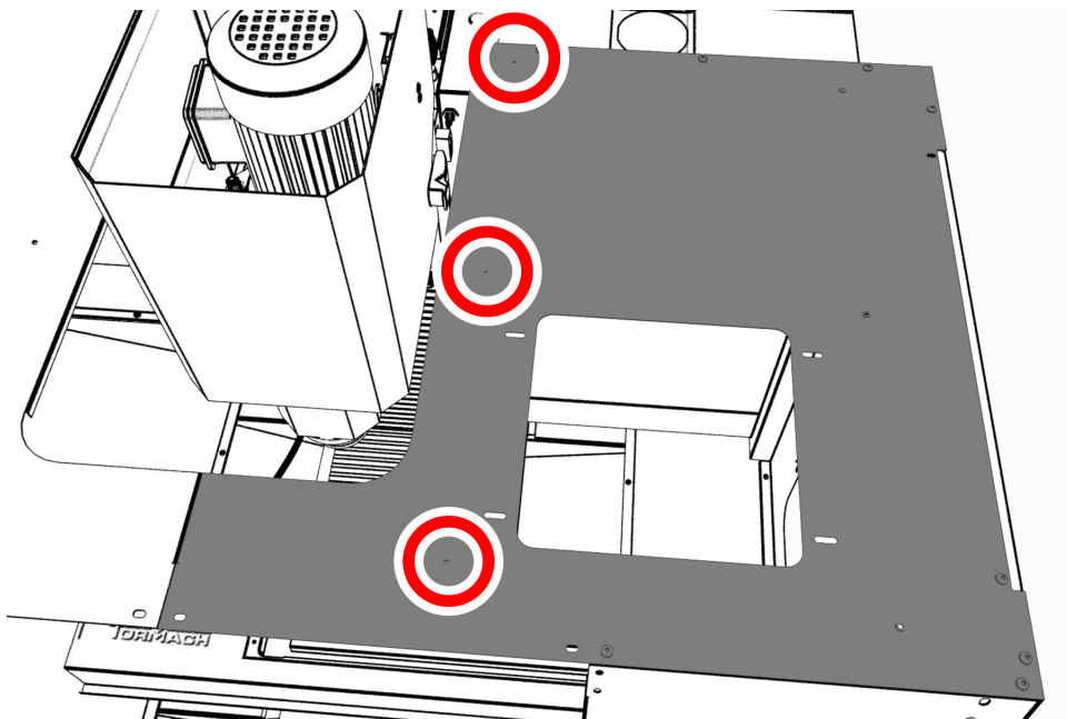
Figure 14: Location to attach three cable tie anchors.
