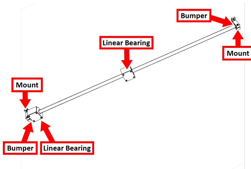
Figure 19: Linear rail assembly.
