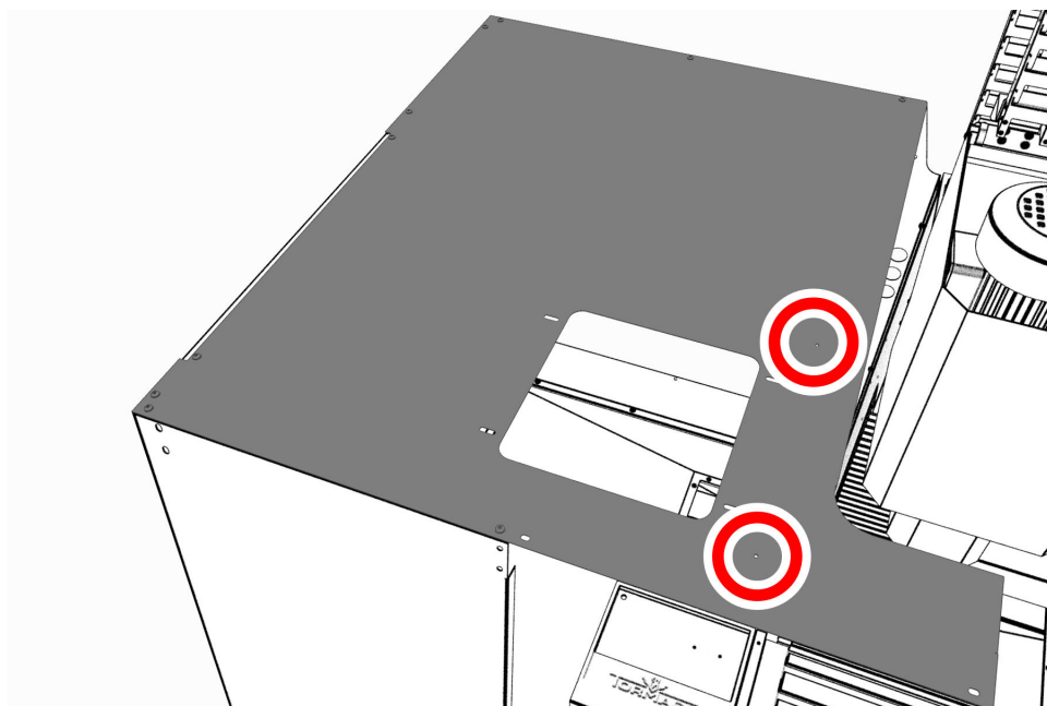
Figure 11: Location to attach two cable tie anchors.
